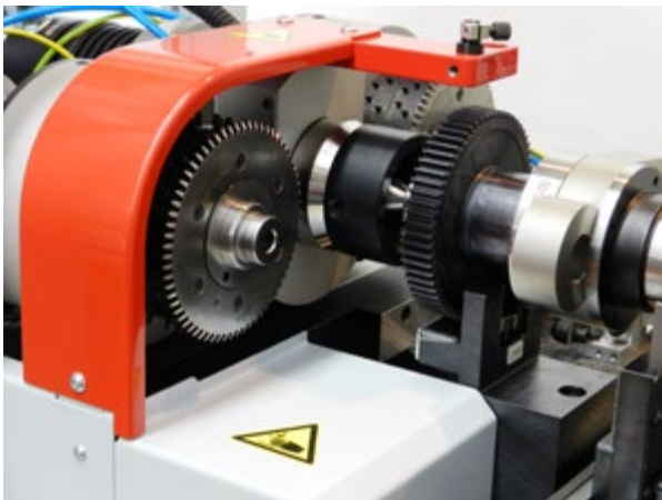
Gear flank analyser with double spindle: cuts measuring time by half
