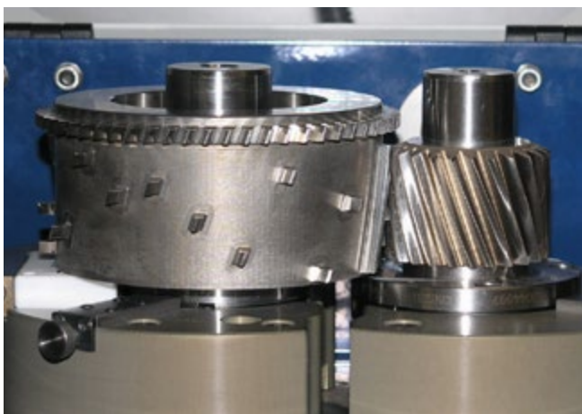
Gear flank analysing with master
