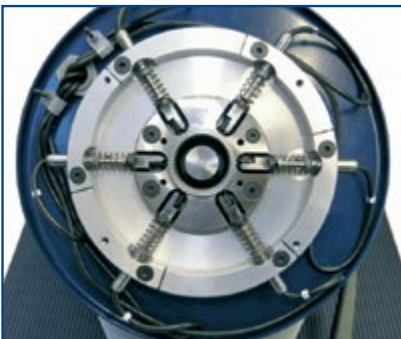
AVM 3x2 RS: 3x2 floating inserts with radius disk
