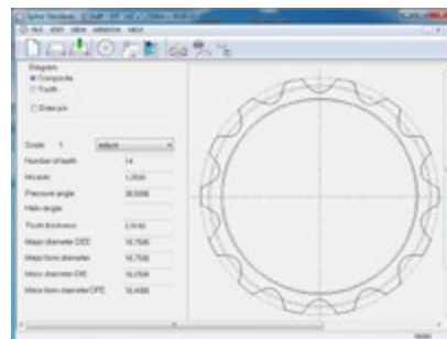
spline profile
