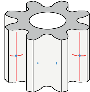
measured profiles, tooth trace and pitch
