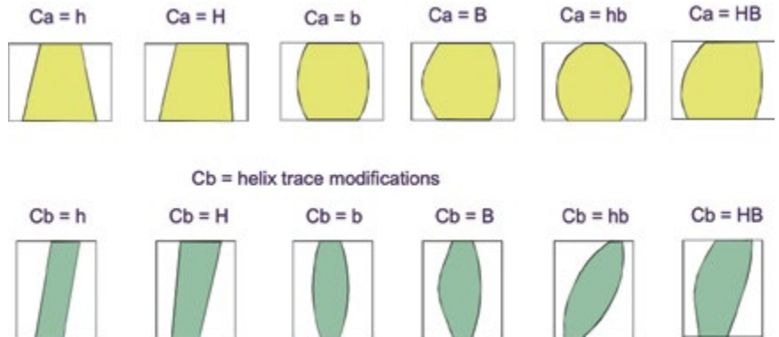
Profile modifications
